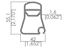
42x55,1 Kumaş Profili 42x55,1 Fabric Support Profile
