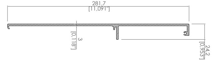
Dere Kapak Profili Gutter Cover Profile
