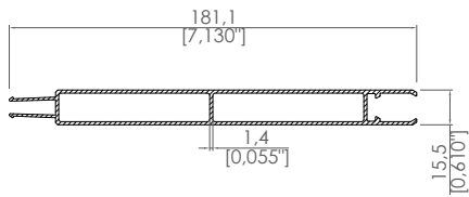
180x15 Panel Profili 180x15 Panel Profile
