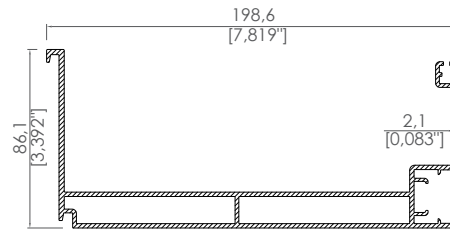
Dere Profili Gutter Profile
